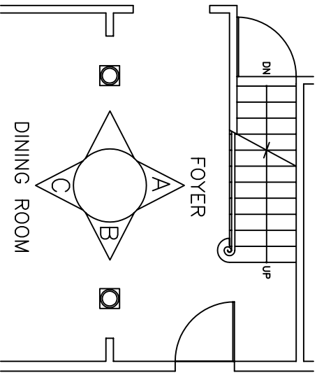
PLAN VIEW
